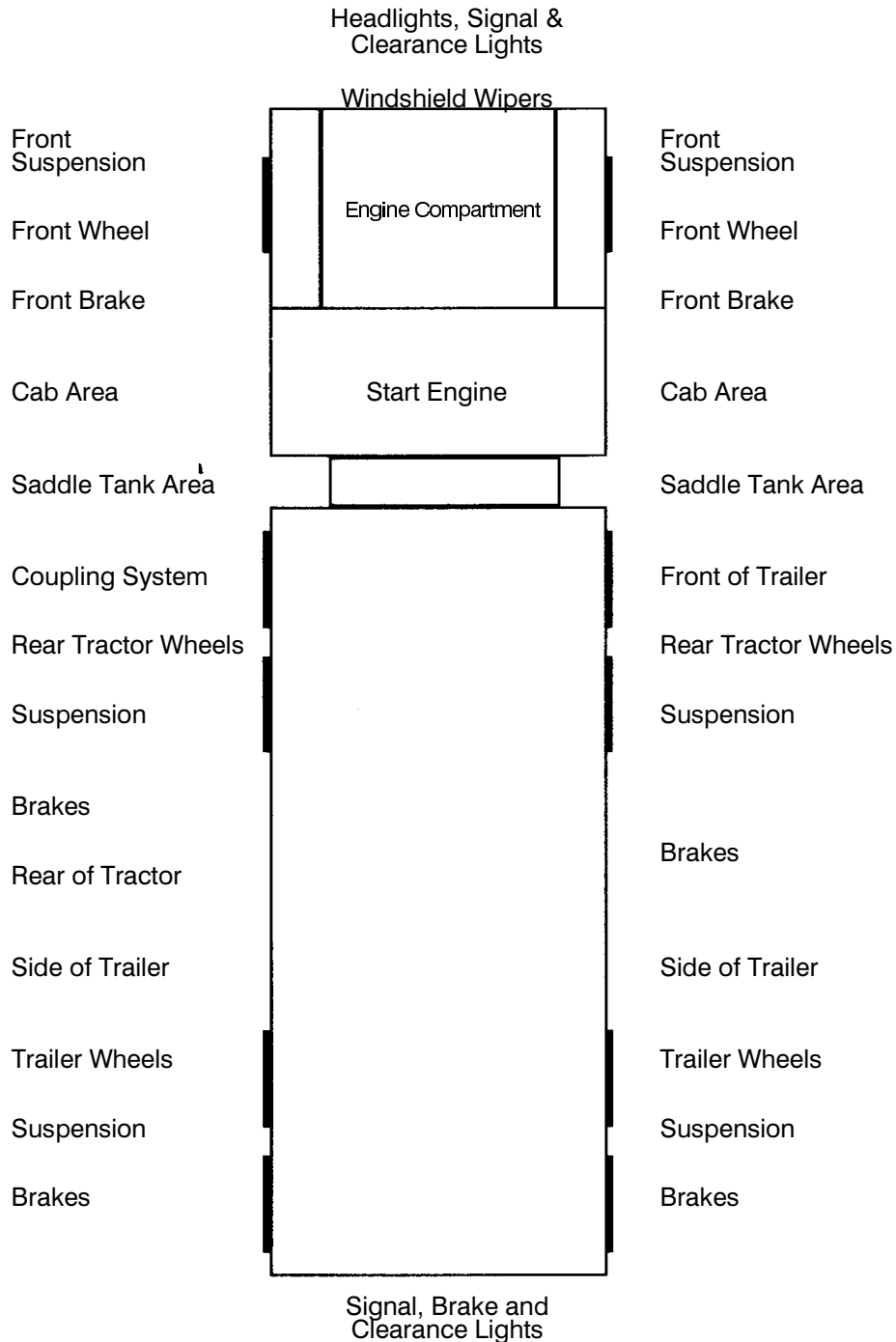
Figure 2-7. Tractor-Trailer
